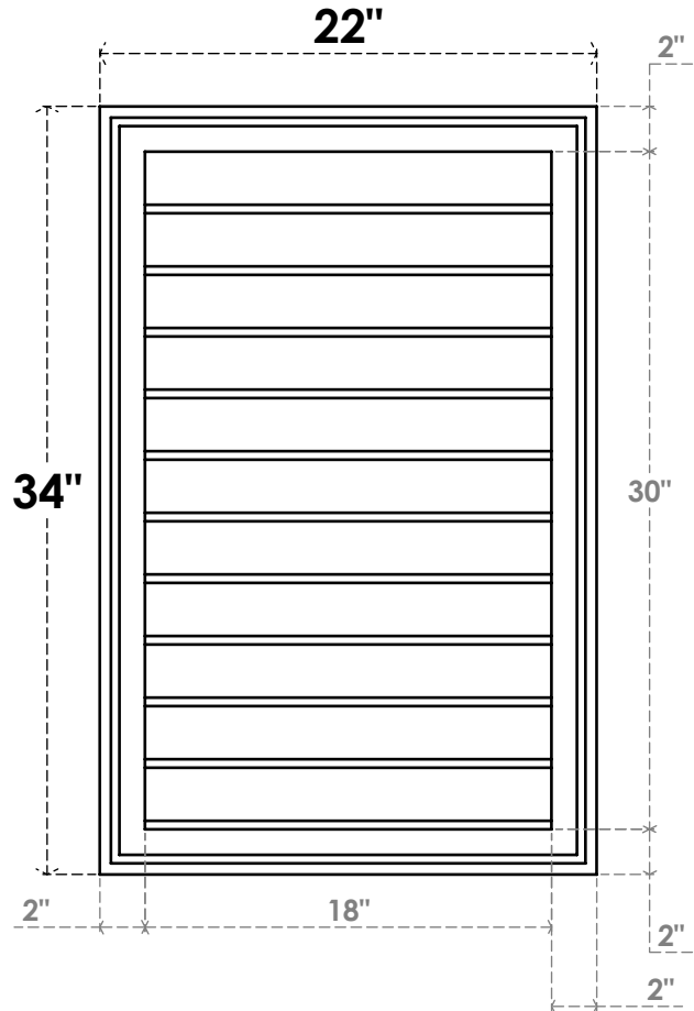
FRONT
